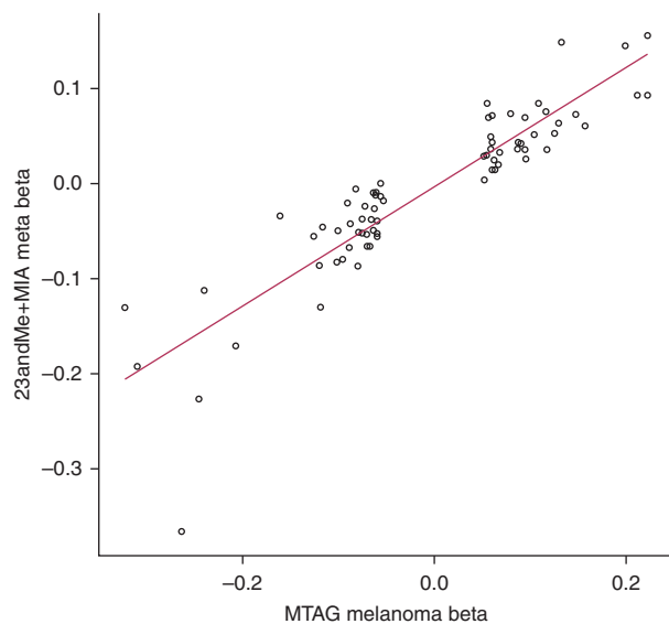
Figure 2. Correlation plot of replication sets and the MTAG melanoma output. For each lead SNP, we plot the corresponding log (OR) effect estimate from the MIA and 23andMe melanoma meta-analysis (Y-axis) against the effect size estimate from the MTAG of melanoma (X-axis). The coefficient of determination ( r^2 ) = 0.81. MIA, Melanoma Institute Australia; MTAG, multitrait analysis of GWAS.
